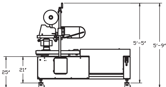
Dimensions shown of base machine only
